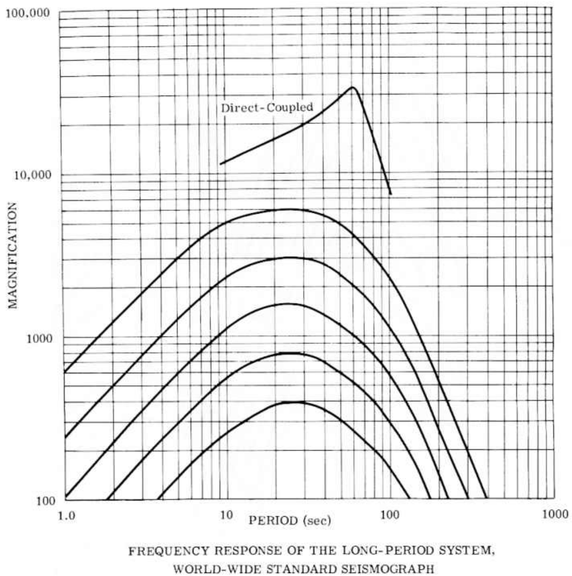
WWSSN Long-Period Instrument Response Curve (from Powell and Fries, 1966)
