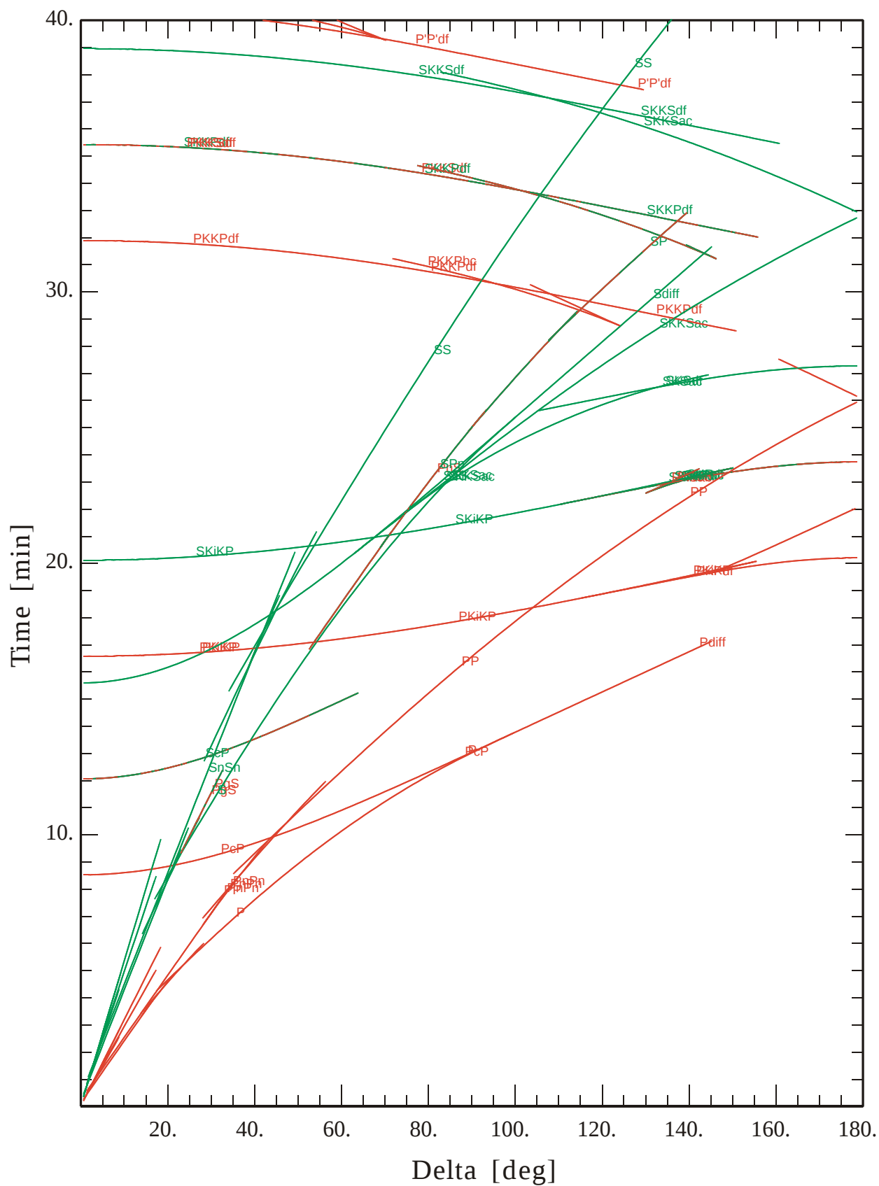
IASPEI '91 Travel Time Curves for shallow events taken from Kennett (1991).
