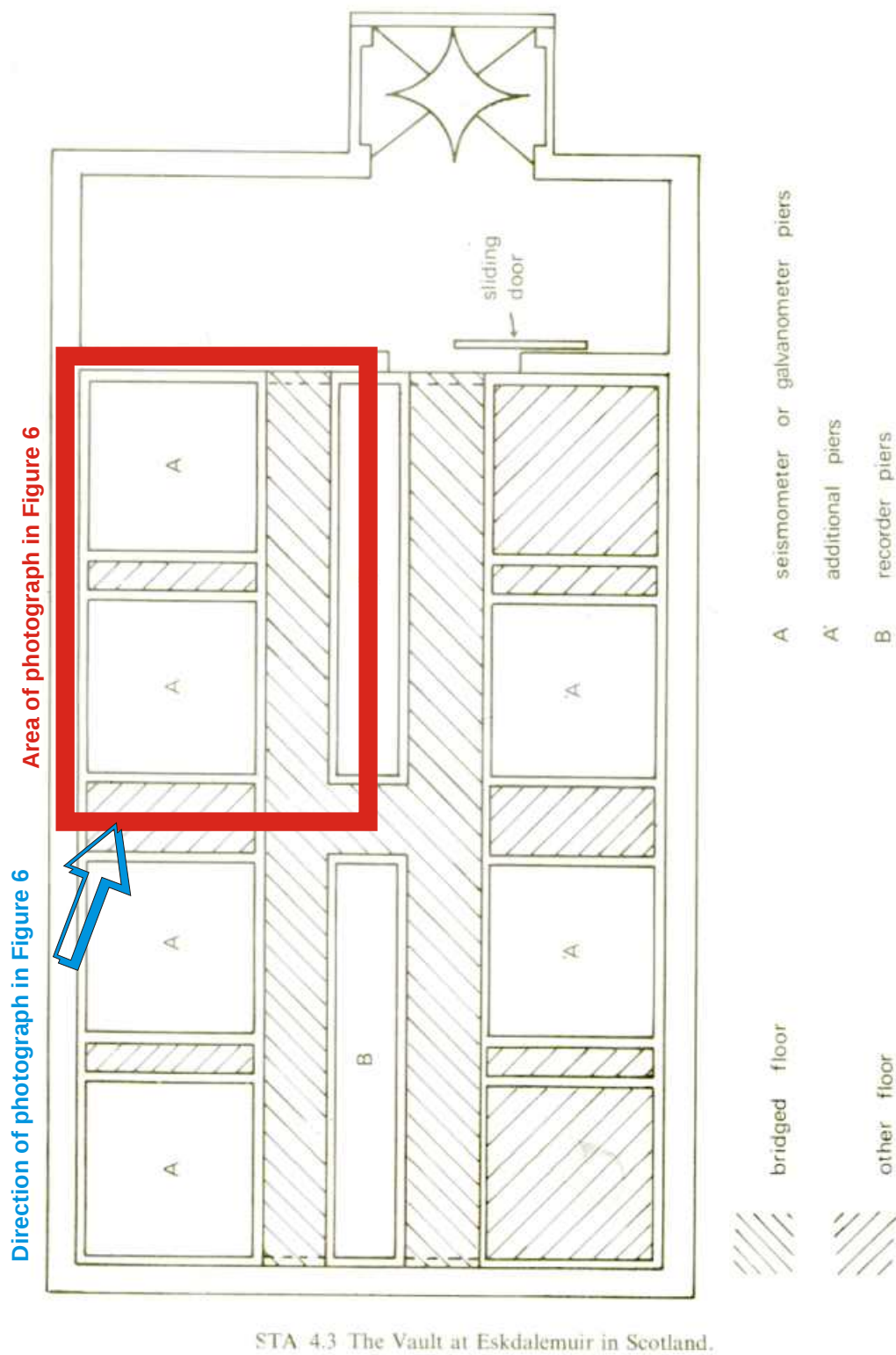
Plan of the ESK WWSSN Station Seismograph Vault (from Powell and Fries, 1966)
