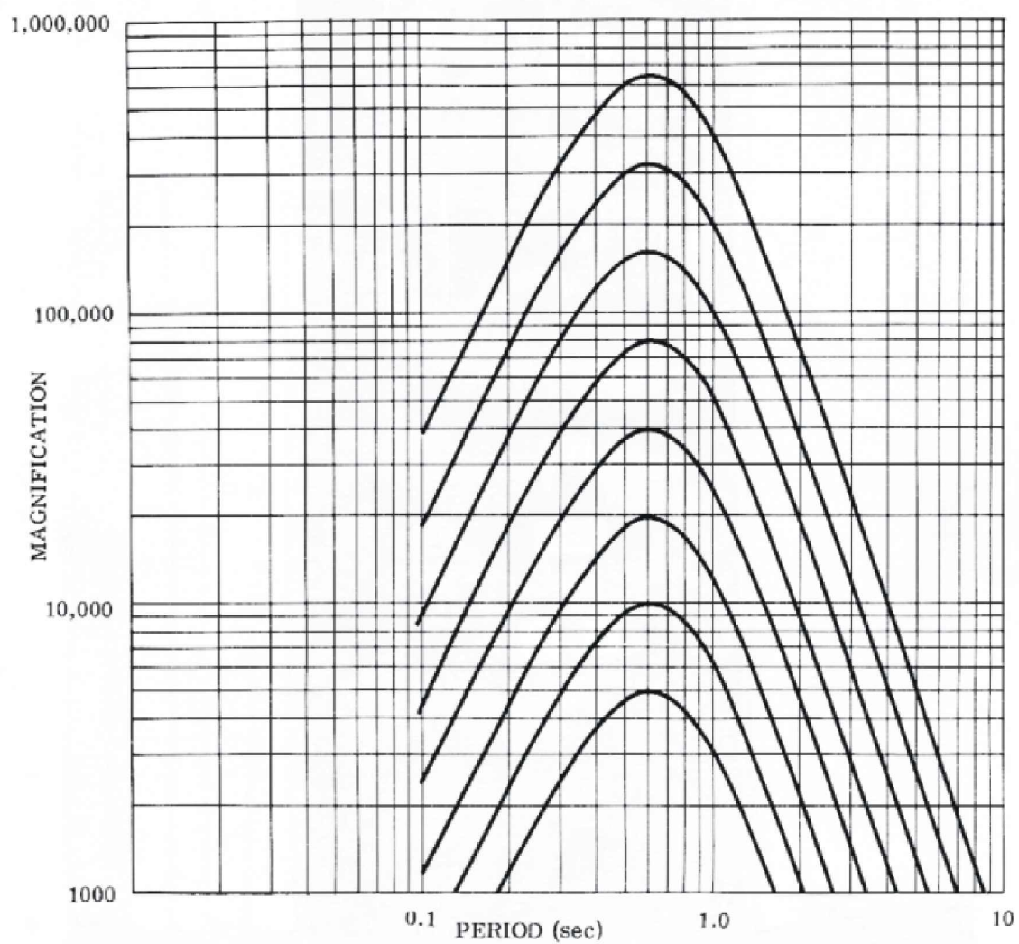
FREQUENCY RESPONSE OF THE SHORT-PERIOD SYSTEM, WORLD-WIDE STANDARD SEISMOGRAPH
