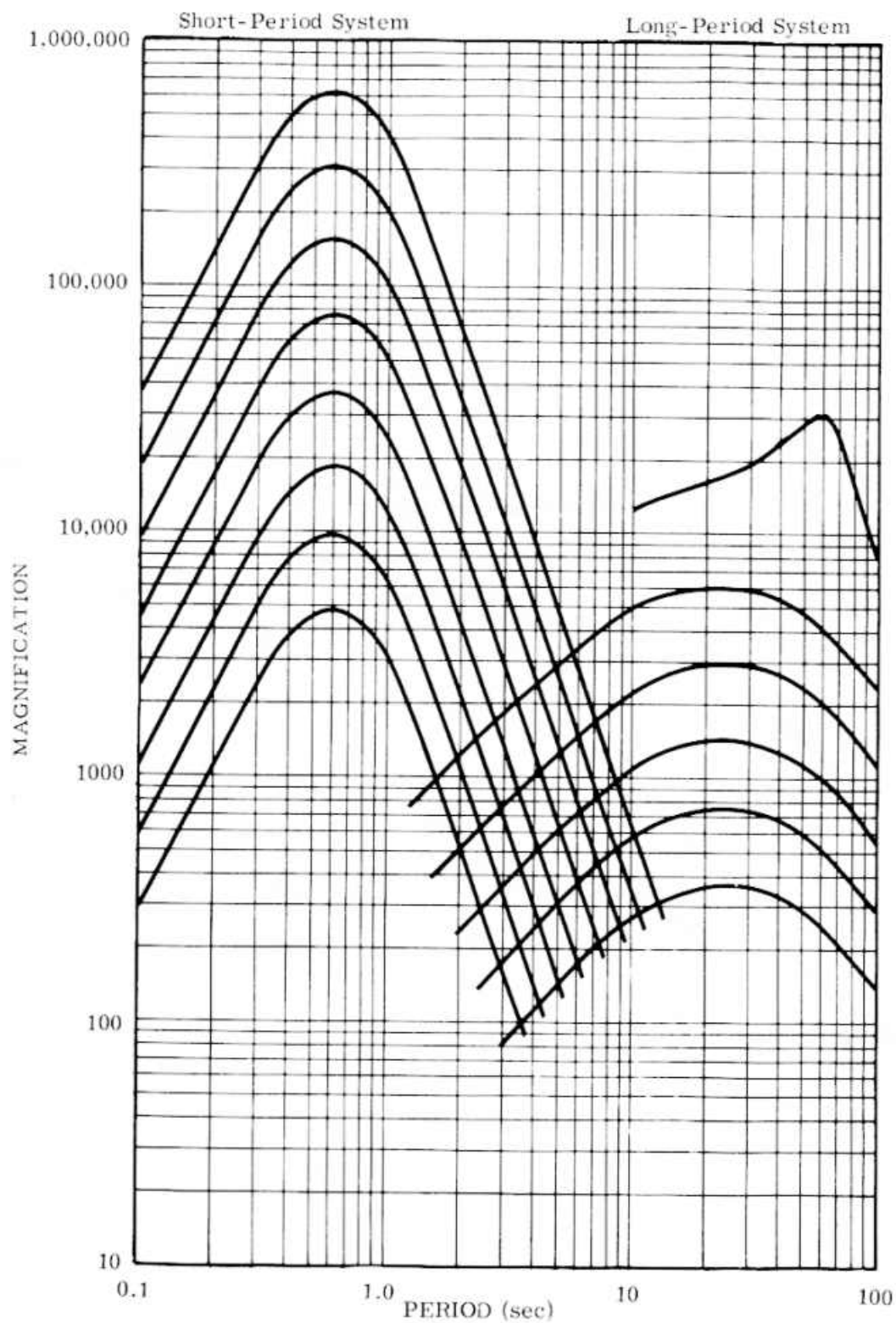
FREQUENCY RESPONSE OF THE WORLD-WIDE STANDARD SEISMOGRAPH
