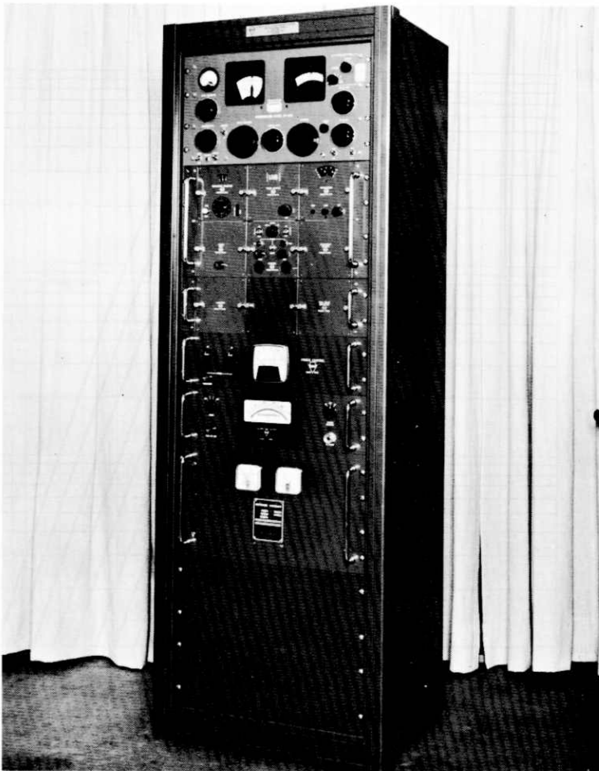
ESK WWSSN Crystal-based Control Console.
